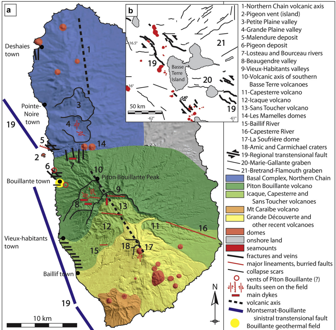
Fig. 2. a) Map summarizing the main structures of Basse Terre Island; b) Regional setting of Basse Terre Island, Guadeloupe Archipelago (modified after Baubron, 1990; Feuillet, 2000; Thion et al., 2010).
