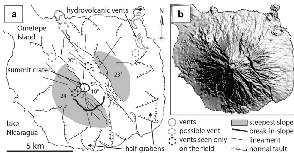
Fig. 3. a) Structural map of Maderas volcano which combines several remote sensing observations (e.g. aerial photography, SRTM, DEM_30 m and field observations). The two upper flank vents (scoria cones) are not visible on remote sensing data and are only documented by field observations; b) DEM_30 m presented as a hill shade map (sun elevation = 45^{\circ} , azimuth = 045^{\circ} ).
