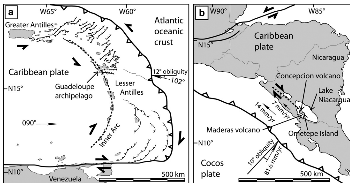
Fig. 1. a) Map of the Lesser Antilles volcanic Arc. The regional tectonic framework is from Feuillet (2000) and the plate motion is from Bouysse et al. (1990), DeMets et al. (2000) and Weber et al. (2001); b) Regional setting of Nicaragua (after Cailleau et al. 2007; DeMets, 2001, van Wyk de Vries, 1993).
