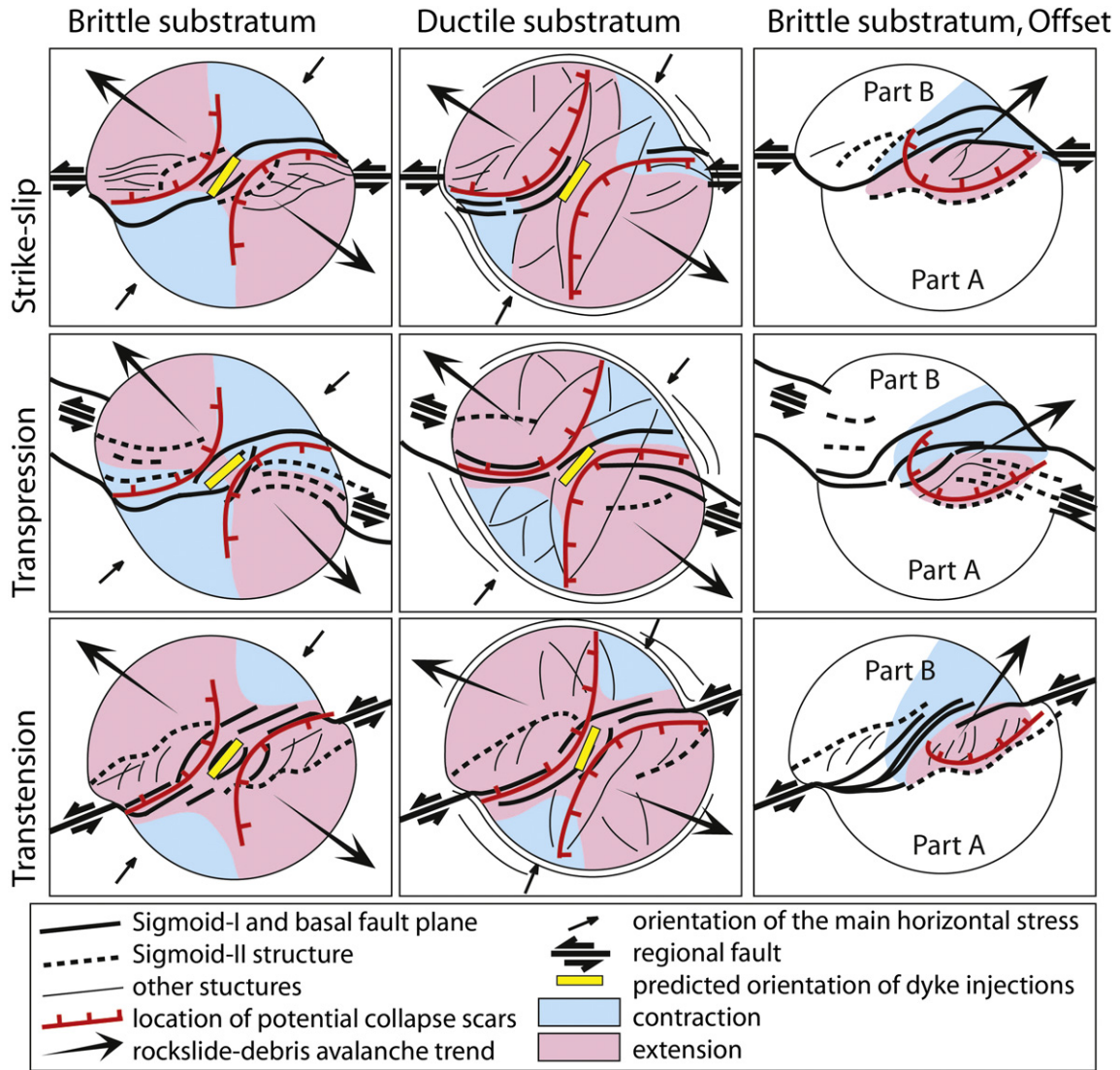
Fig. 4. Sketches summarizing the likely location of dykes and collapse scars in cones that develop in the vicinity of sinistral strike-slip, transtensional and transpressional fault zones.
