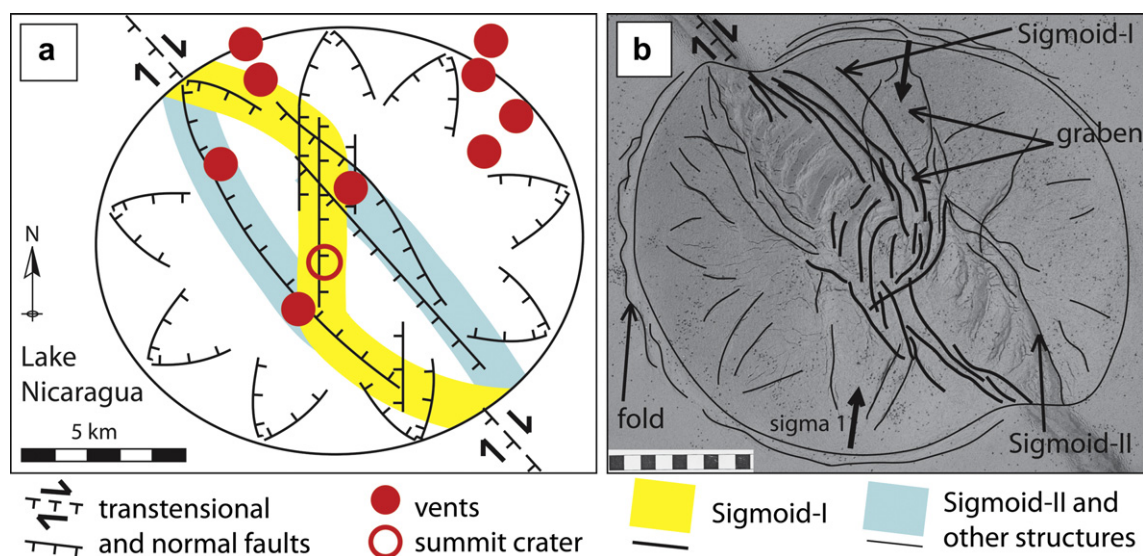
Fig. 6. a) Structural sketch of Maderas volcano, Nicaragua. Note that the exact location and throw direction of the regional fault zone are unknown; b) Picture of experiments C19 (dextral transtensional fault, \alpha = 20^\circ , brittle and ductile substratum).
