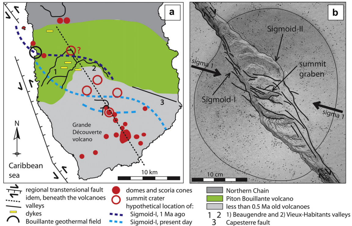
Fig. 5. a) Structural sketch of the southern part of Guadeloupe Island, Lesser Antilles; b) Picture of experiment C33 (sinistral transtensional fault, \alpha = 20^\circ , brittle substratum).
